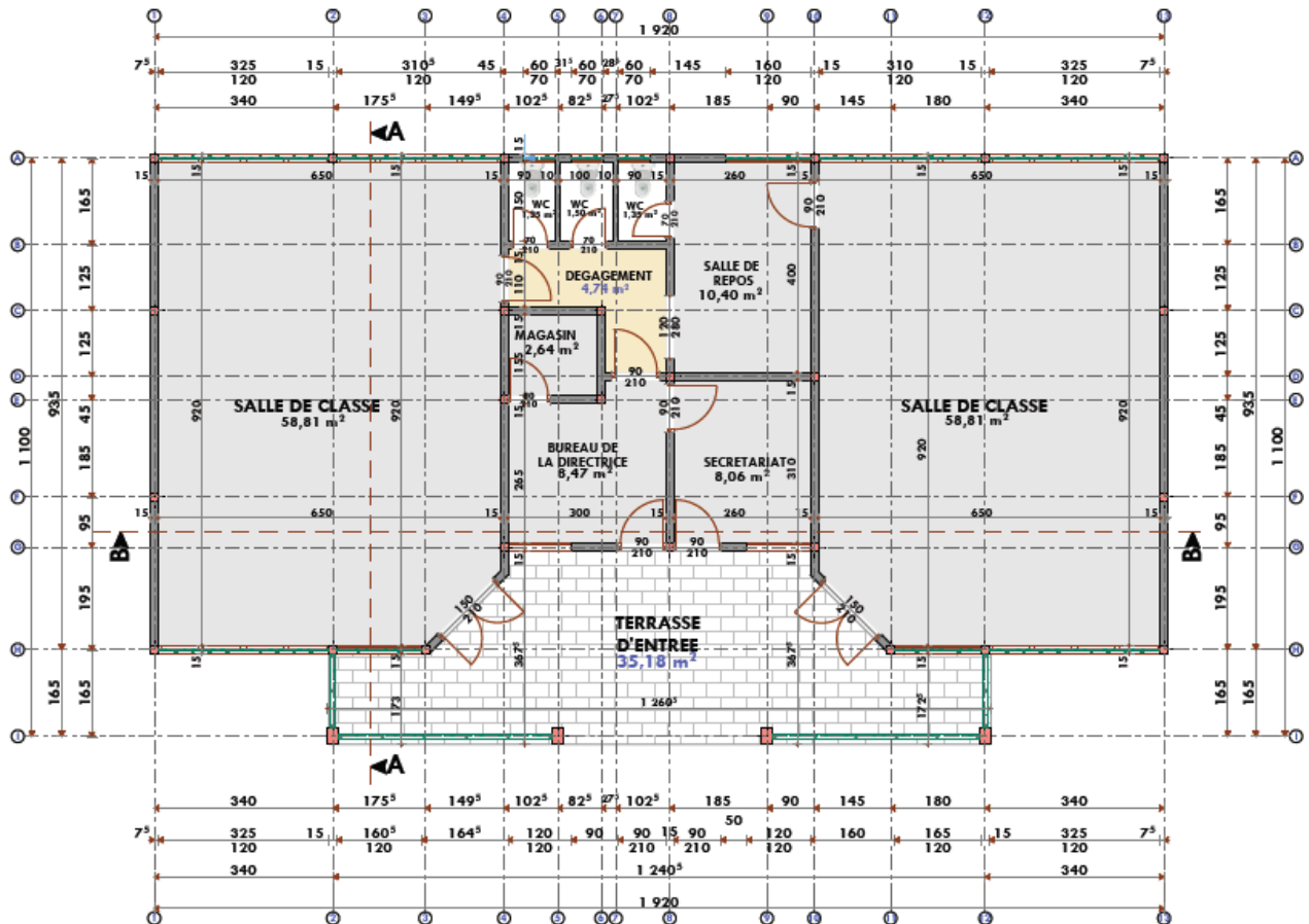
PLAN DE DISTRIBUTION - DISTRIBUTION PLAN
